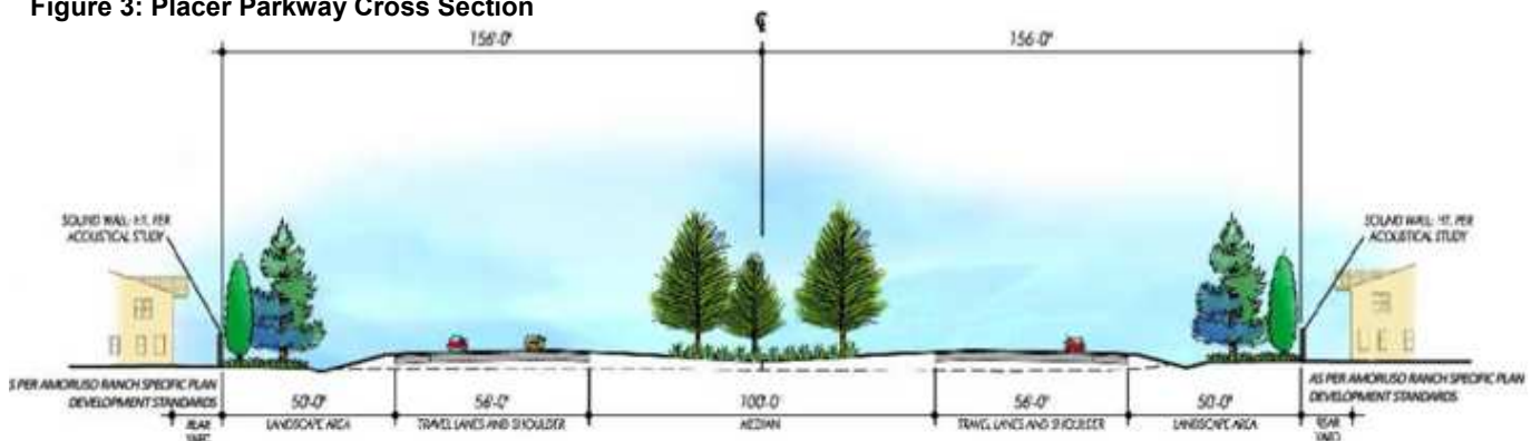
Figure 3: Placer Parkway Cross Section
